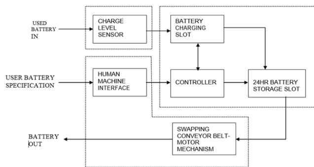
.2.BASIC BLOCK DIAGRAM OF BSS
