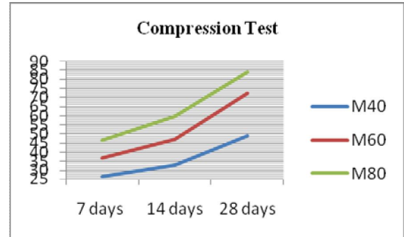
Figure No. 3 Compression Result
