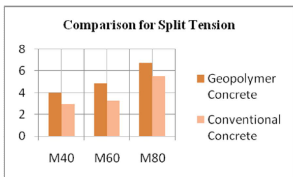
Figure No. 6 Comparison of Tension Result
