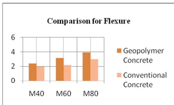
Figure No. 7 Comparison of Flexure Result
