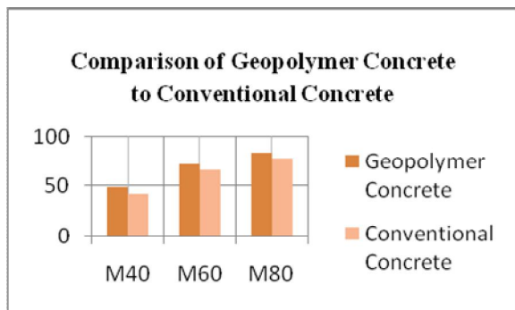
Figure No. 5 Comparison of compression Result
