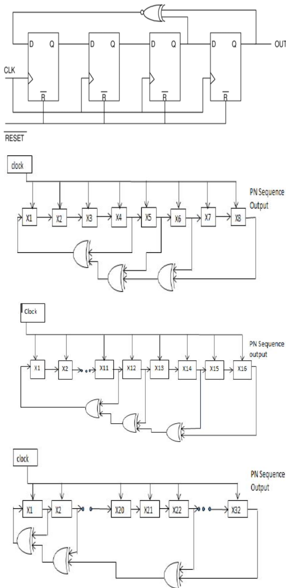
Figure 1: General block diagram of LFSR
