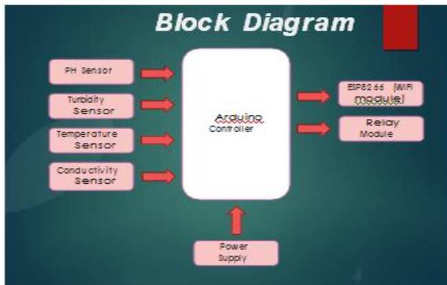
Figure 2. Water Quality Monitoring System
