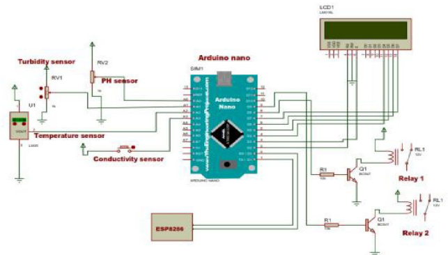
Figure 1. Water Quality Implementation System
