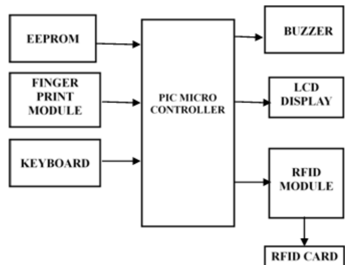
Fig 3 Block Diagram
