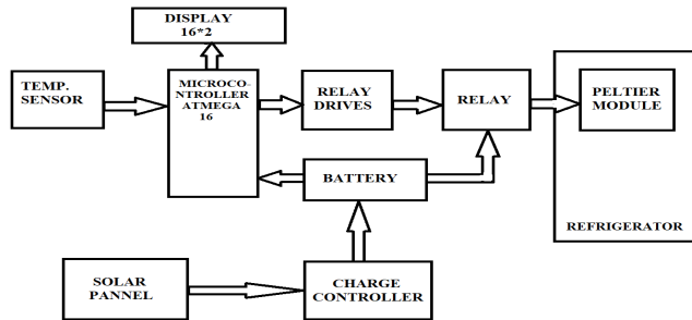
Figure. Block diagram solar based refrigeration system
