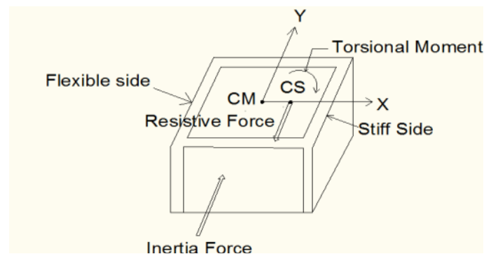
Fig 1 Generation of torsional moment in asymmetric structures
