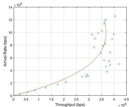
Fig.1 Throughput versus Packet arrival rate at receiving station
