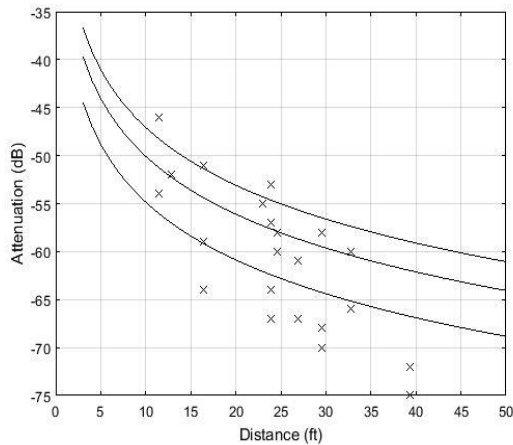
Fig.3 Fading in signal strength with respect to distance with colliding packets
