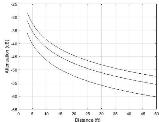
Fig.2 Fading in signal strength with respect to distance without colliding packets
