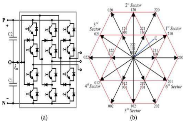
Fig.1. Typical three-level inverter (a) structure of circuit, and (b) three-level.
