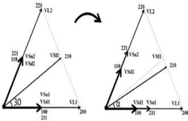
Fig. 4. Vector diagram in the first sector of Fig. 1(b) showing the change of the vectors using balanced dc and unbalanced dc assuming V_{c1} < V_{c2} . inverter under both balanced and unbalanced capacitor voltages.
