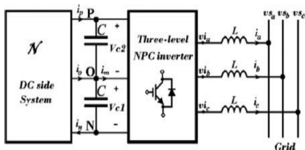
Fig.3. General diagram of a grid connected three-wire three-level inverter.
