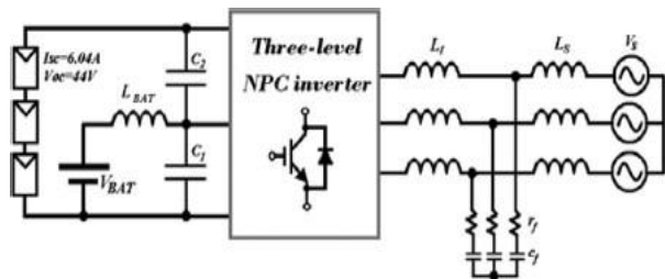
Fig. 8. Block diagram of the simulated system.
