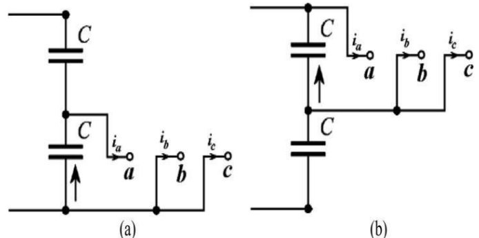
Fig.2. Equivalent circuit and capacitors current with two different short vector. (a) Short vector—100. (b) Short vector—211.
