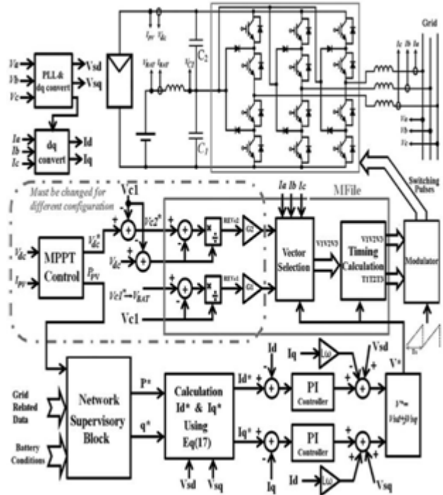
Fig.7. Control system diagram to integrate PV and battery storage.
