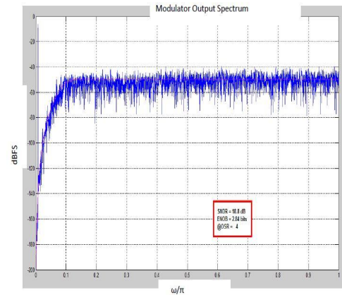
Fig.5 Frequency Domain Simulation Of Fourth Order Sigma Delta Modulator With CIBF Architecture
