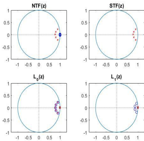
Fig.6 Stability Analysis of 5 th Order Filter
