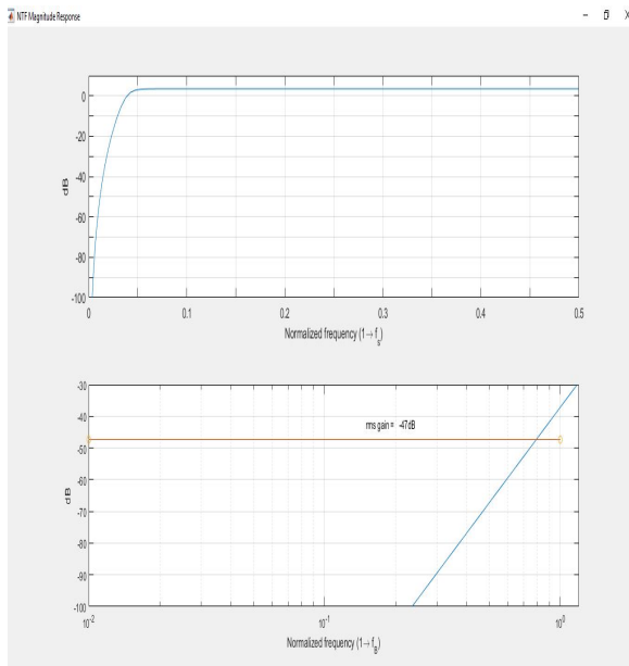
Fig.7 Stability Analysis of 5 th Order Filter
