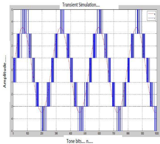
Fig.3 Time Domain Simulation Of Fourth Order Sigma Delta Modulator With CIBF Architecture
