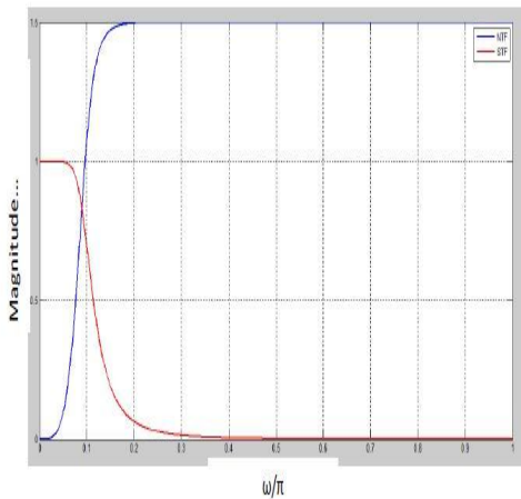
Fig.2 Realization of STF and NTF in voltage
