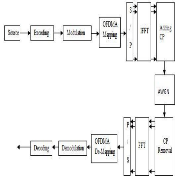
Fig.1 Block Diagram of WiMAX Transceiver[7]
