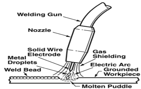
Fig 1 GAS METAL ARC WELING
