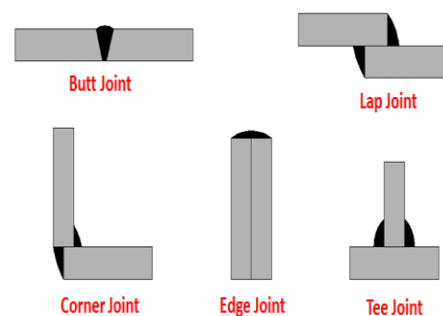
Figure.1.2: Types of welding joints
