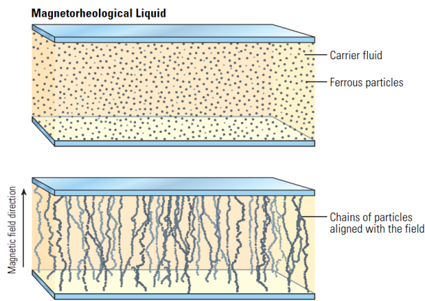
Fig 1.2(a) chain like structure formation in controlable fluid
