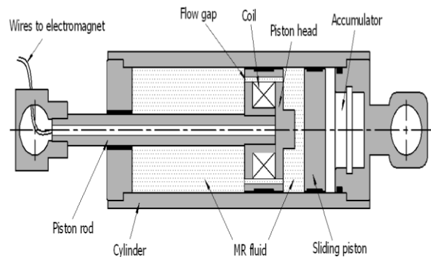
Fig.1.1 Magnetorheological Damper
