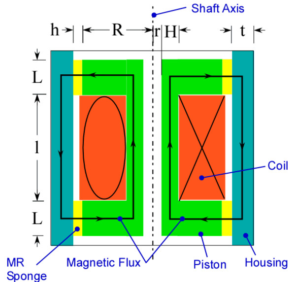
Fig.3.1 Dimensions of MR Fluid Damper
