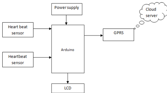
Block diagram of Proposed system
