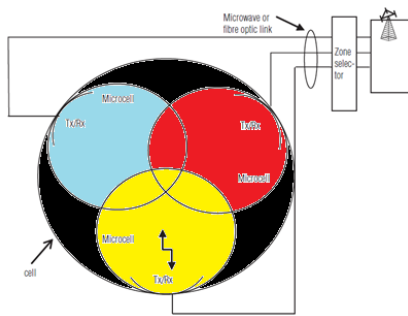
Fig-4 Microcell zone concept (for three microcells)
