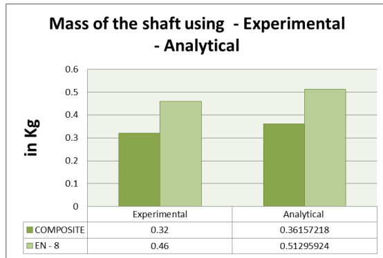
Graph 1 . Comparative of Mass FOR both Shafts in Experimental and Analytical
