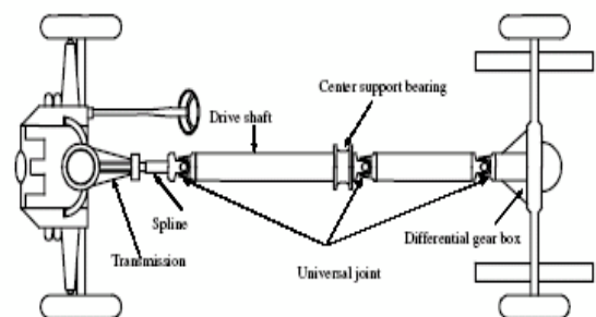
Figure 1: Two-piece Drive shaft present in a Driving system.
