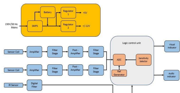
Fig. 1. System Level Block Diagram
