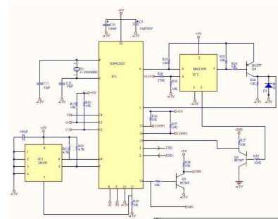
Fig. 8. Microcontroller Interface
