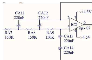
Fig. 5. 3 rd order Sallen-key Low Pass Filter
