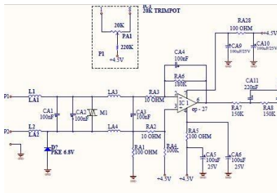
Fig. 6. First Gain Stage
