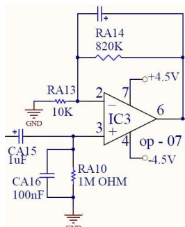
Fig. 7. Second Gain Stage
