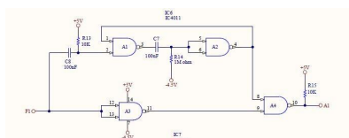
Fig. 3. Digital Filter
