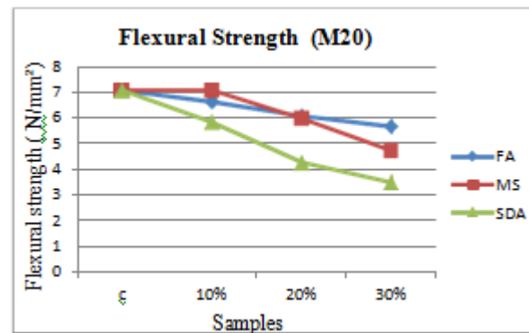
Fig 7. Flexural strength for egg shell powder with admixtures (28 days)
