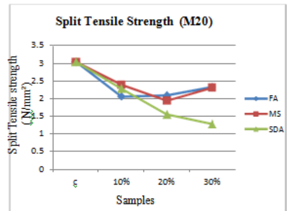
Fig 8. Split tensile strength for egg shell powder with admixtures (28 days)
