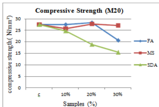
Fig 6. Compressive strength for egg shell powder with admixtures (28 days)
