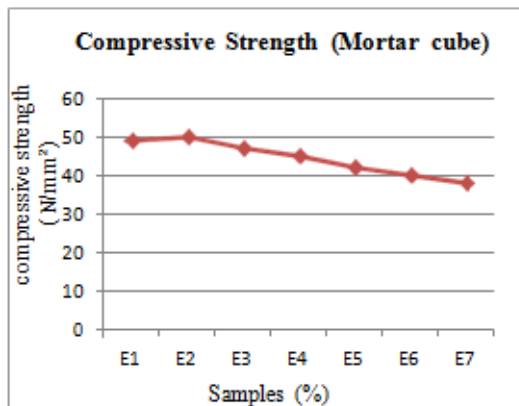
Fig 5. Compressive strength for egg shell powder (28 days)
