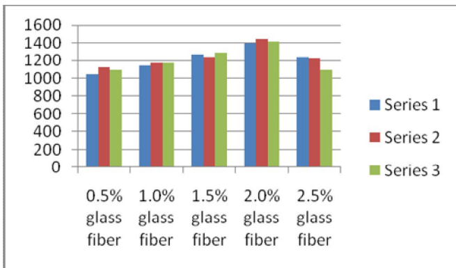
Figure.3 stability values for 0.1% of Zycotherm in bitumen
