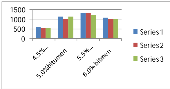
Figure1. Stability values for different mix proportions of bitumen (for OBC)
