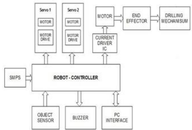
Fig. 3 Proposed System
