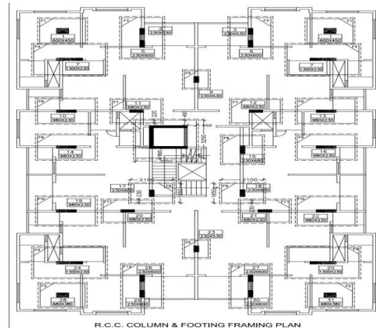
Fig 13: R.C.C. COLUMN & FOOTING FRAMING PLAN
