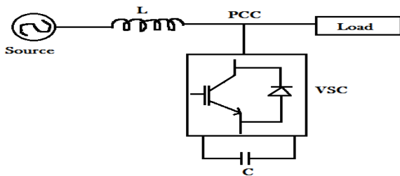
Fig 2:-STATCOM Model
