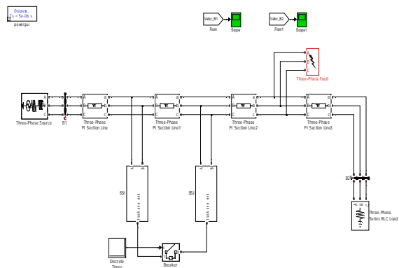
Fig 1:- Electrical Railway traction feeding system
