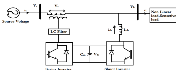
Fig 3:-UPQC Model
