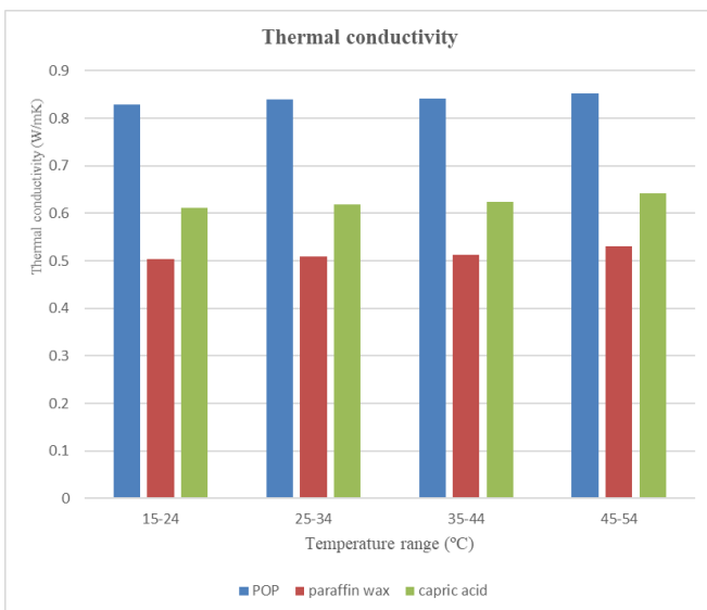
Chart 7.1 Thermal conductivity trend of POP samples
