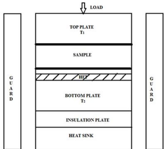
Fig. 6.4 Arrangement of apparatus.
