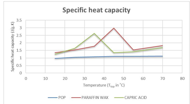
Chart 7.2 Specific heat capacity versus temperature plot.
