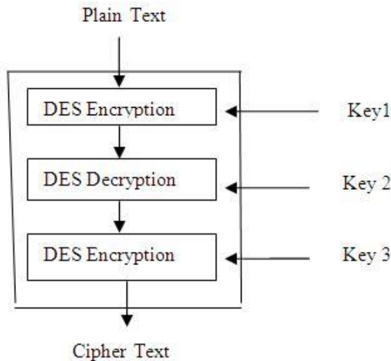
Figure 3.2: Encryption in 3DES
