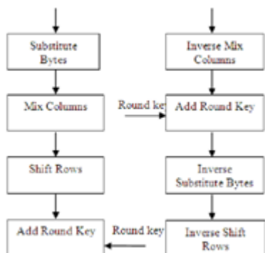
Figure 3.3: One Round of encryption and Decryption in AES
