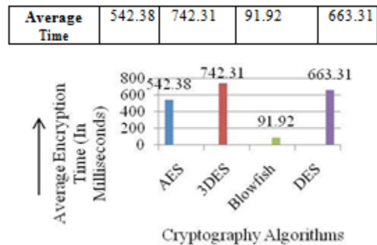
Figure 2: Encryption Time of Each Algorithm (In ms)
