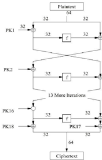
Figure 3.4: Blowfish Encryption
