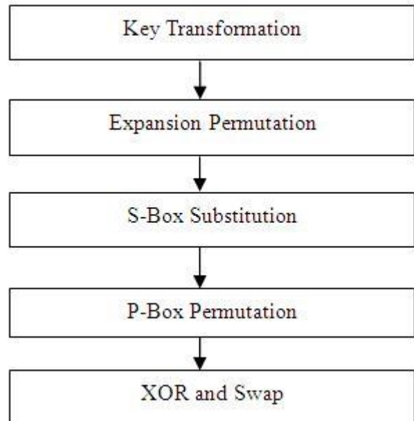
Figure 3.1: Details of One Round in DES
