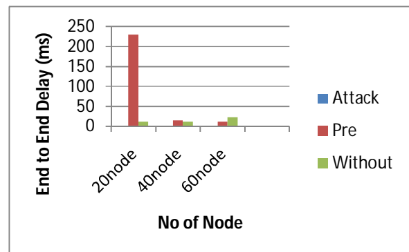
Figure.2: End To End Delay under Attack, Pre and Without
