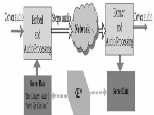
Figure 1.1 Block diagram for audio steganography[9]
