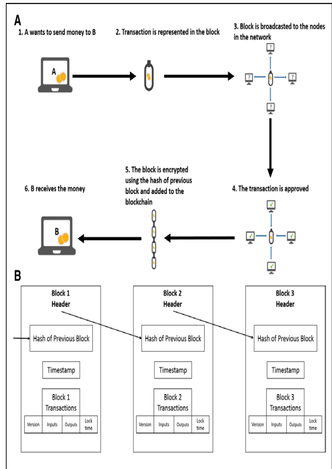
Figure. The execution of a transaction in blockchain (A) and the representation of a block in the blockchain (B).
