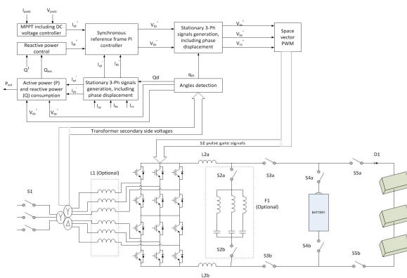
Figure 2: Control block diagram of R12SC circuit
