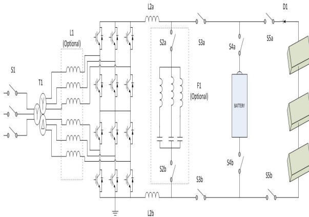
Figure 1: Schematic diagram of the proposed R12SC Circuit
