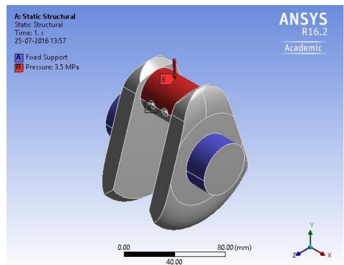
Fig modelling of Crankshaft by Cad Tool and Finite Element Analysis Using Ansys Software
