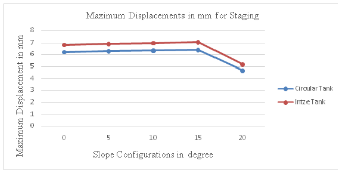
Graph 6.3 Maximum Displacements in circular tank and Intze tank
