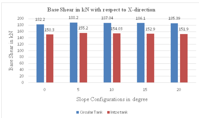
Graph 6.1 Base Shear in kN with respect to X-direction
