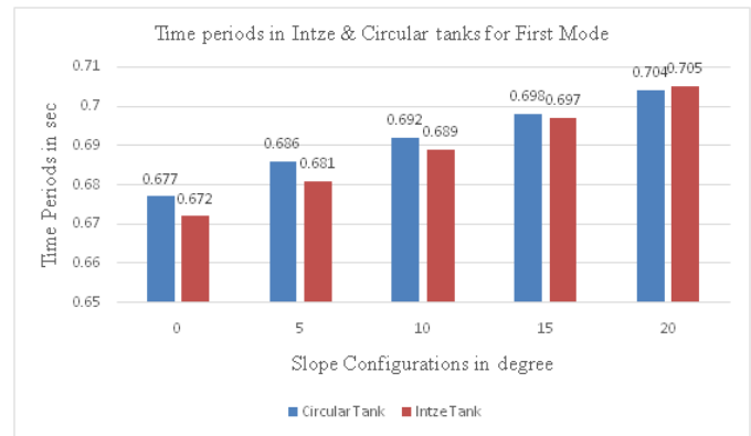
Graph 6.4 Time periods in Circular tank and Intze tank
