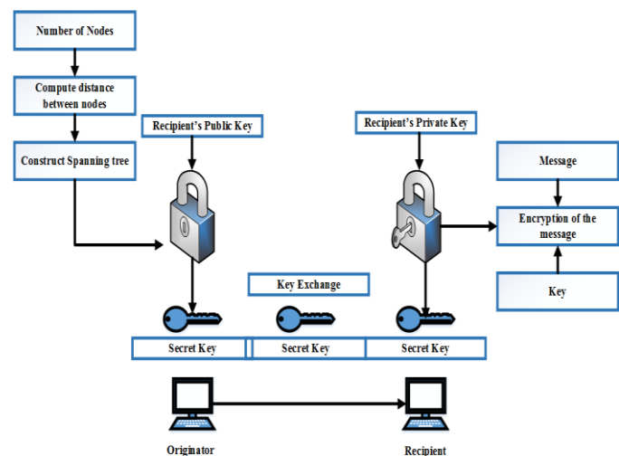
Figure 2 Key management architecture Khalil et al., (2008)
