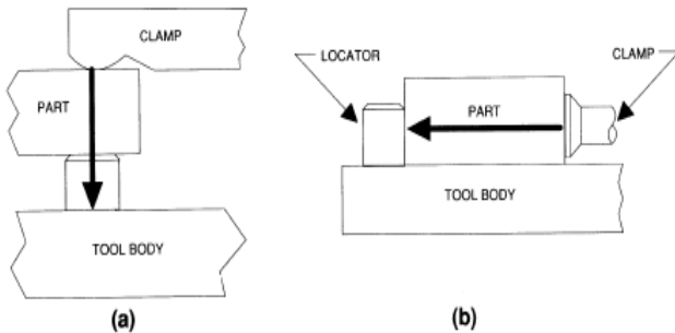
Figure 1. Locators.[5]
