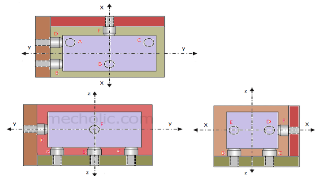
Figure 3. 3-2-1 Location principle.[5]
