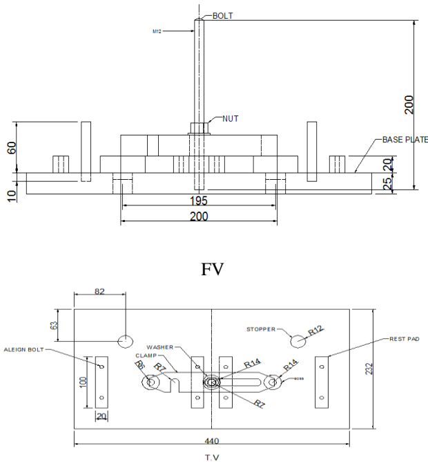
Figure 5. 2D Drawing of fixture.
