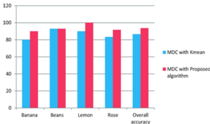
Fig. 8. Classification results per class for proposed method.
