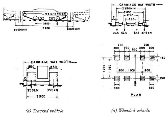
Fig 3.1 IRC Class AA loading
