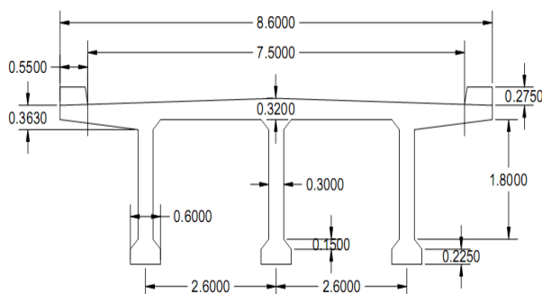
Fig 4.2 Cross Section of Bridge
