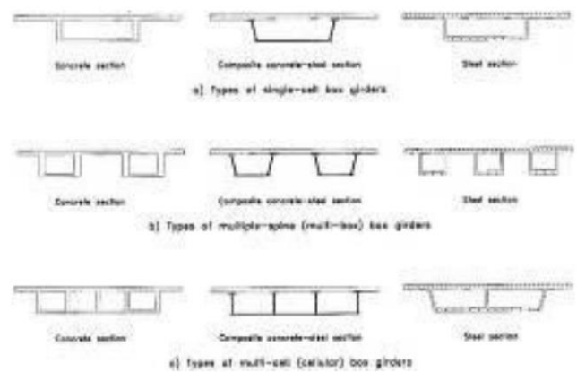
Fig1.3: Types of girder
