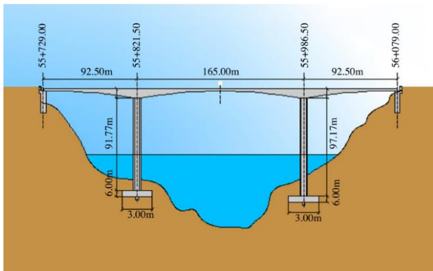
Fig1.1: The Budan Bridge and its dimensions.
