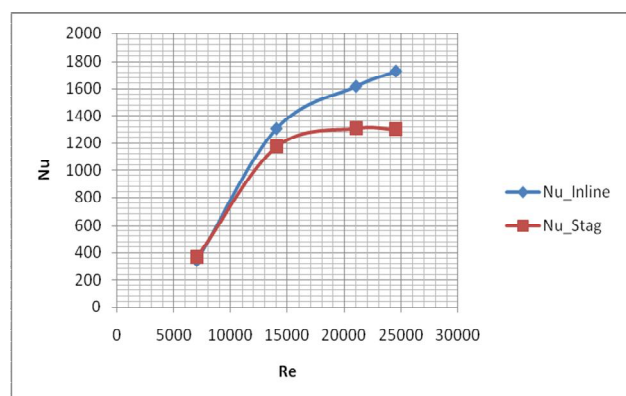
Fig. 6 Variation of Nusselt Number to Reynolds Number.
