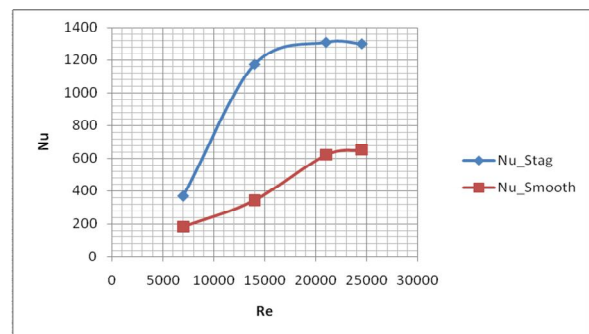
Fig. 5 Variation of Nusselt Number to Reynolds Number.
