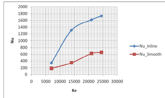
Fig. 4. Variation of Nusselt number to Reynolds Number.
