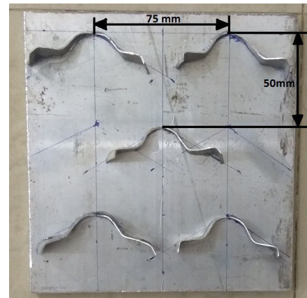
Fig.4 Staggered wavy delta winglet on flat plate
