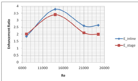
Fig.7 Variation of enhancement factor to Reynolds Number.
