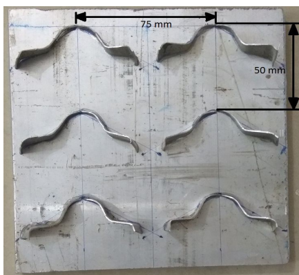
Fig.3.Inline wavy delta winglet on flat plate
