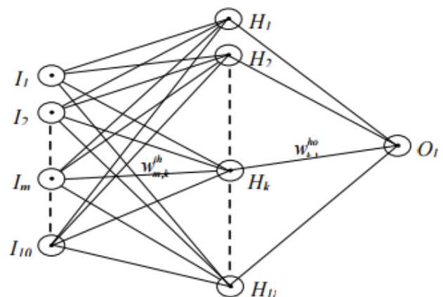
Figure 2. Configuration of the developed neural network (12-12-1)
