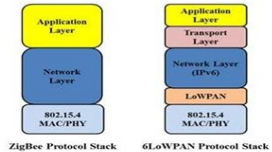
Figure 2: 6LoWPAN and ZigBee protocol stack [35]
