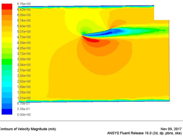
Fig 5 Contour 1 velocity contour with 15 degree flange
