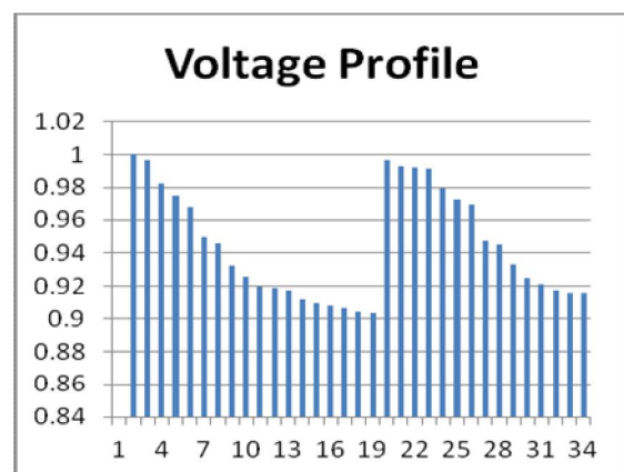
Voltage profile Of IEEE 33 Bus system
