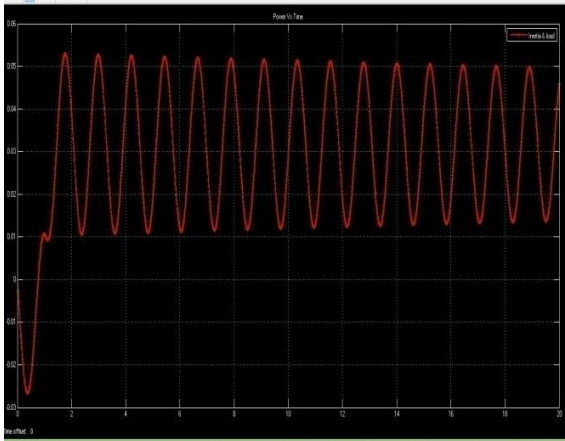
Figure 4 Response for open loop single area Change in power It is found from graph that with open loop if demand changes to 0.2 pu, a steady state error exists in frequency of 0. Close Loop AGC for Single Area System
