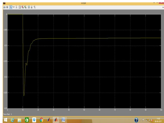
Fig 17 Response for Area 1 AGC system for change in frequency
