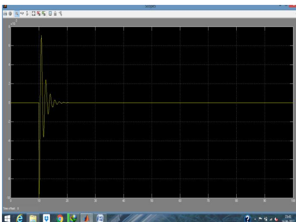
Fig 33 performance graph of change in power in area 3 using FLC
