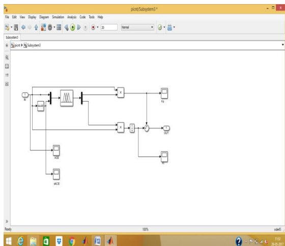
Fig 27 Simulink Model of fuzzy logic controller with PI in MATLAB
