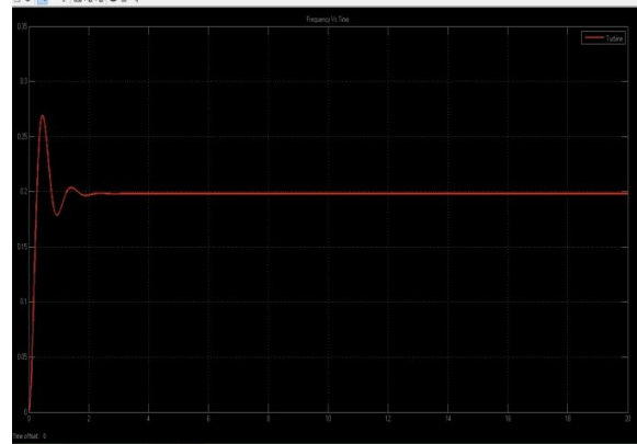
Figure 6 Response for close loop AGC system for change in frequency
