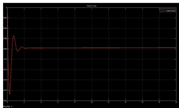
Figure 7 Response for close loop AGC system for change in power
