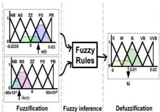
Fig.1. Fuzzy Inference system for FLC
