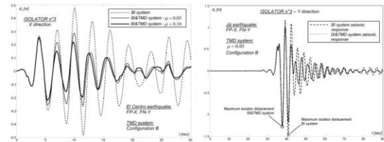
Figure 2: TMD effectiveness in reducing base isolators relative displacement
