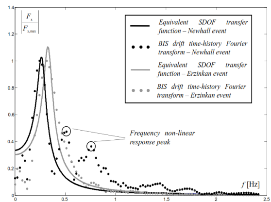
Figure 5: Equivalent SDOF to model the isolators’ frequency non-linear response
