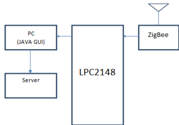
Fig. 2. Working of Distribution end system
