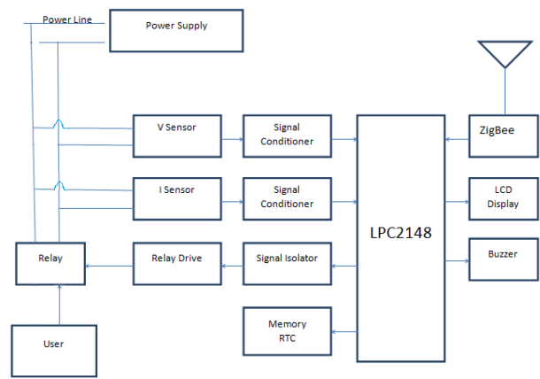
Fig 1. proposed User end system
