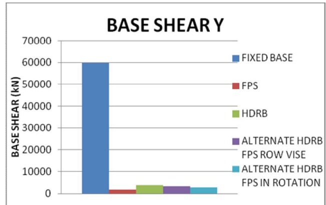
Base Shear in Y-Direction
