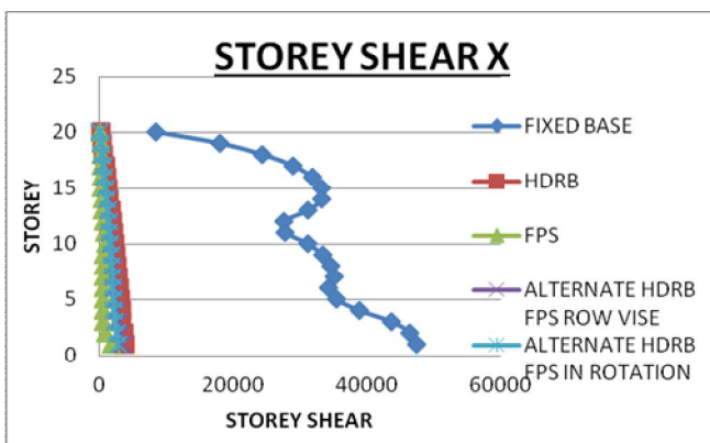
Storey Shear in X-Direction
