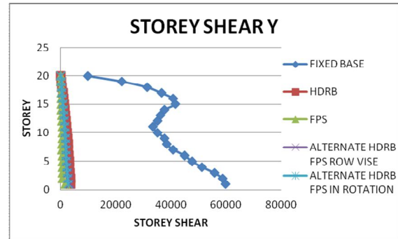
Storey Shear in Y-Direction
