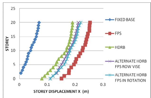
Storey Displacement in X-Direction
