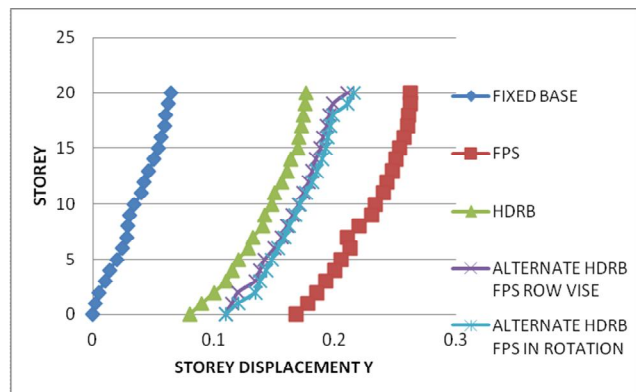
Storey Displacement in Y-Direction
