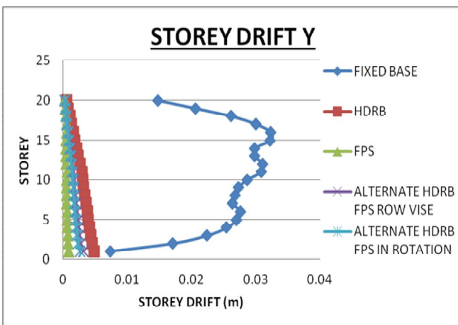
Storey Drift in Y-Direction
