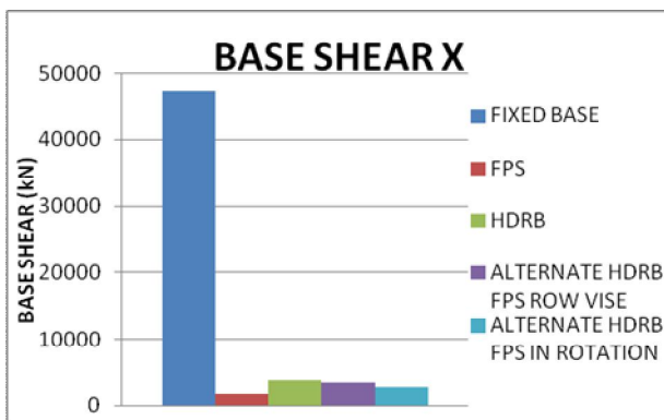
Base Shear in X-Direction
