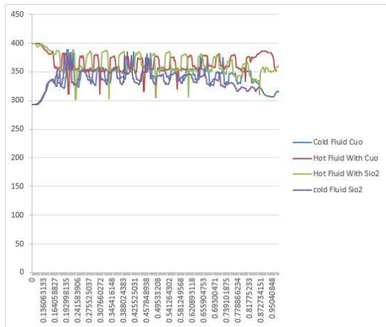
Figure 19: Temperature Distribution of Cold Fluid and Hot Fluid in CuO and SiO 2 along the length of the plate
