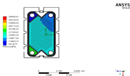
Figure 7: Pressure Distribution of the Fluids along the plate heat exchanger using Cold Fluids
