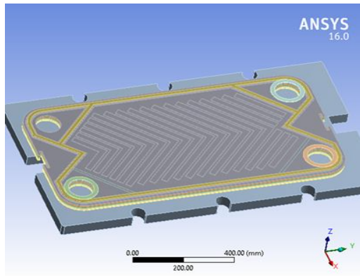
Figure 4: Mesh
