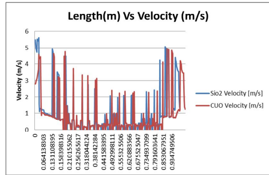
Figure 17: Velocity comparison along the length of the plate with nanofluids
