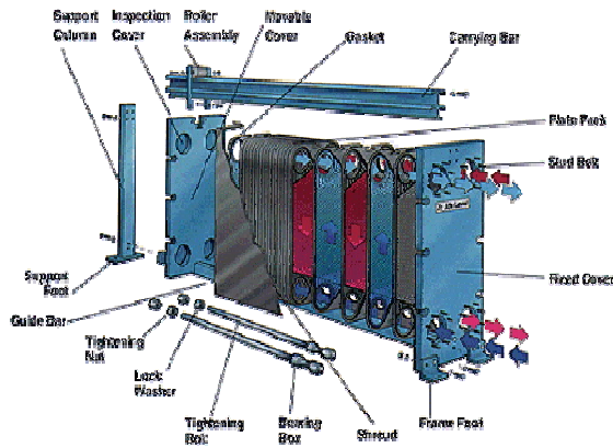
Figure 1: Gasketed plate and frame exchanger (courtesy Mueller).
