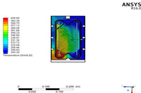
Figure 6: Temperature Contour with Water
