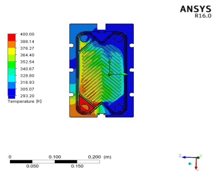
Fig 13: Temperature Distribution on the plate heat exchanger using CuO nanofluid
