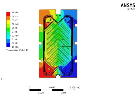
Figure 10: Temperature Distribution on the plate heat exchanger using SiO 2 nanofluid
