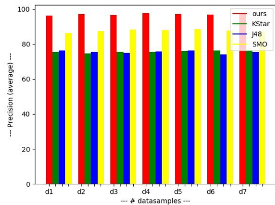
Fig 2: Average precision graph
