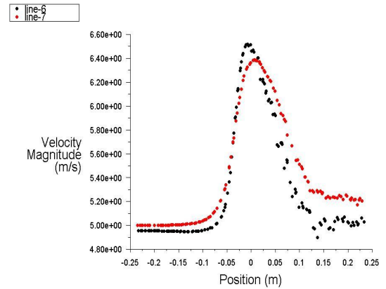
Velocity Magnitude Nov 11, 2017 ANSYS Fluent Release 16.0 (2d, dp, pbns, ske)
