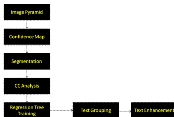
Figure: Flow of Proposed Work
