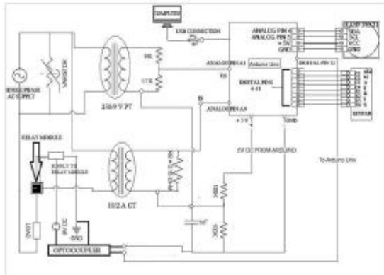
(Fig. 1 – Circuit Diagram of the Prototype)
