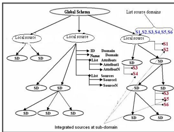
Figure 2: Integration Tree structure
