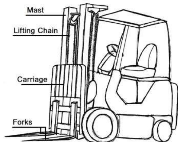
Fig.forklift mechanism
