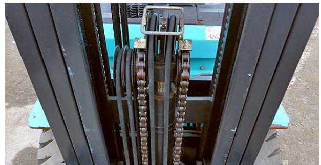
Fig. Chain mechanism
